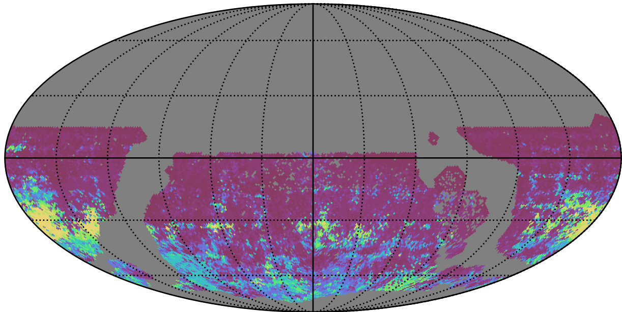
too_elab_heavy_r64_d3_ugrizy_v3.4_10yrs WFD r band: 75th Percentile Intranight Timespan
