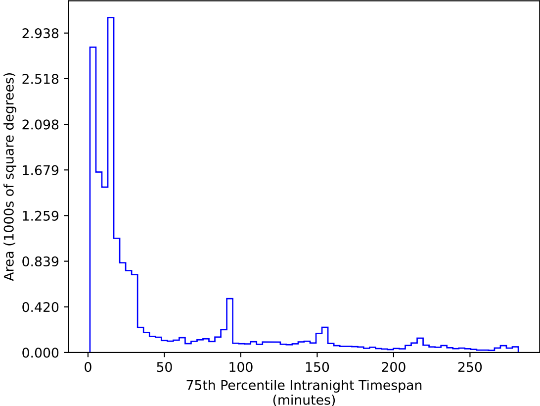
too_elab_heavy_r64_d3_ugrizy_v3.4_10yrs WFD r band: 75th Percentile Intranight Timespan
