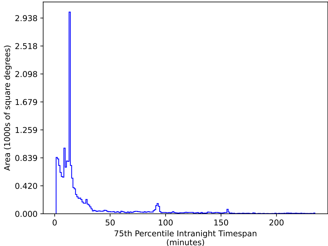
too_elab_heavy_r64_d3_ugrizy_v3.4_10yrs WFD i band: 75th Percentile Intranight Timespan
