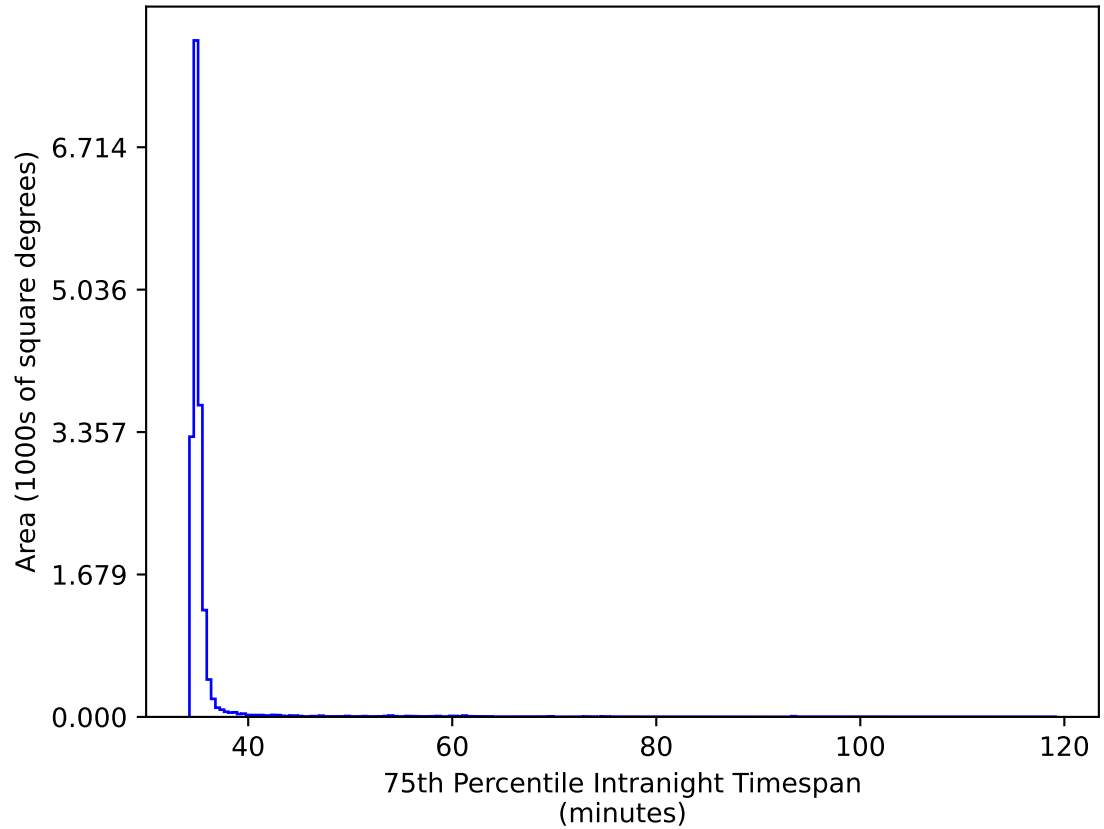
too_elab_heavy_r64_d3_ugrizy_v3.4_10yrs WFD gr bands: 75th Percentile Intranight Timespan
