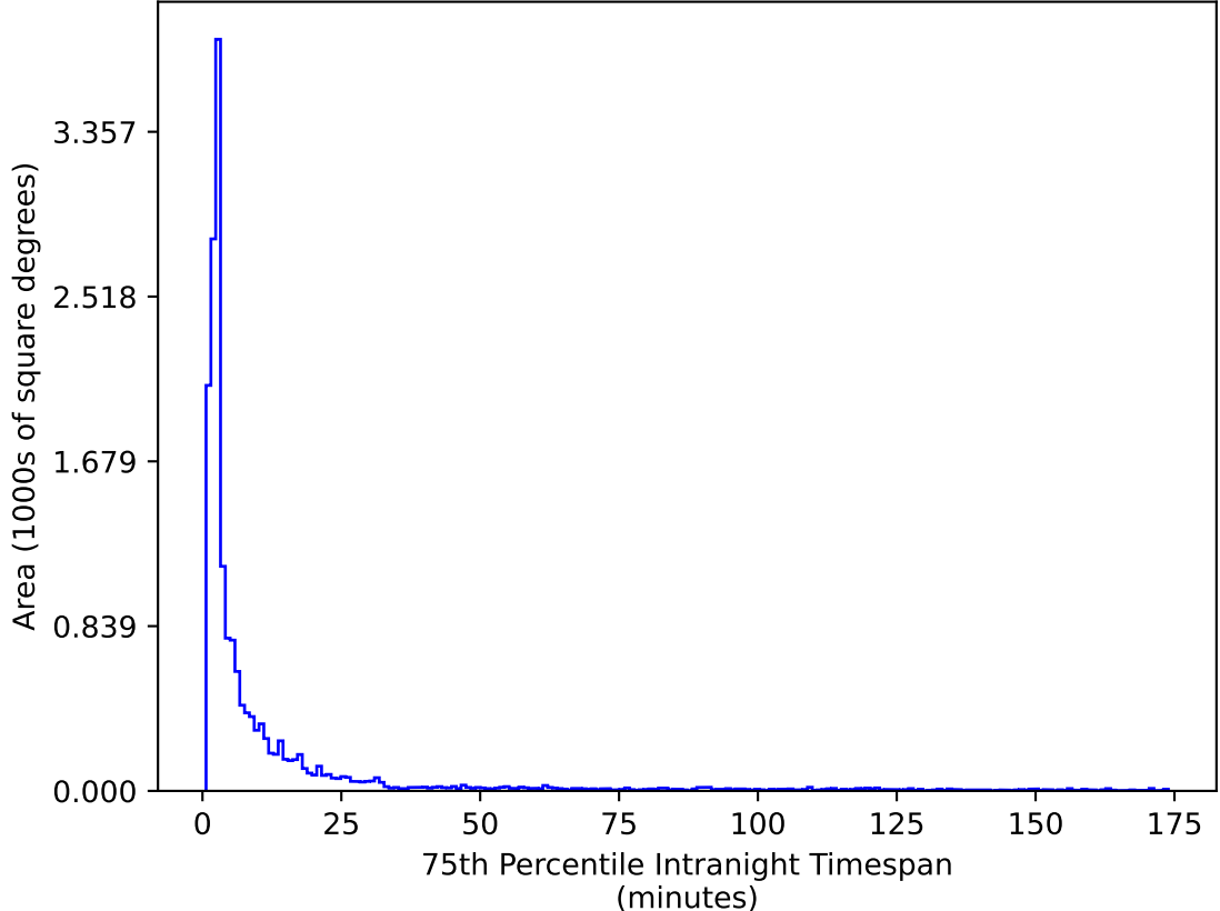
too_elab_heavy_r64_d3_ugrizy_v3.4_10yrs WFD g band: 75th Percentile Intranight Timespan
