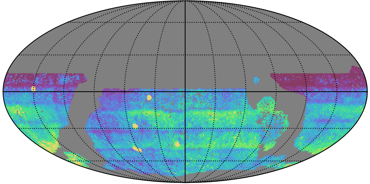
too_elab_heavy_r64_d3_ugrizy_v3.4_10yrs WFD all bands: 75th Percentile Intranight Timespan
