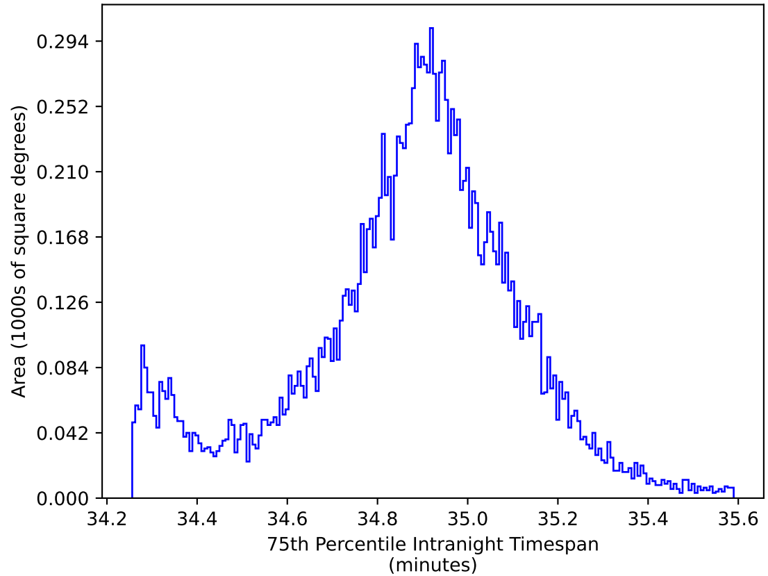
too_elab_heavy_r64_d3_ugrizy_v3.4_10yrs WFD all bands: 75th Percentile Intranight Timespan
