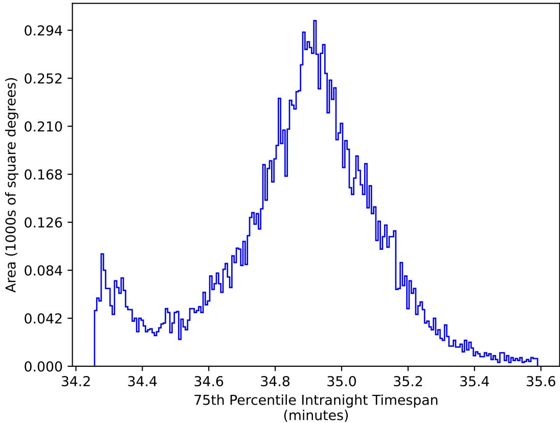
too_elab_heavy_r64_d3_ugrizy_v3.4_10yrs WFD: 75th Percentile Intranight Timespan
