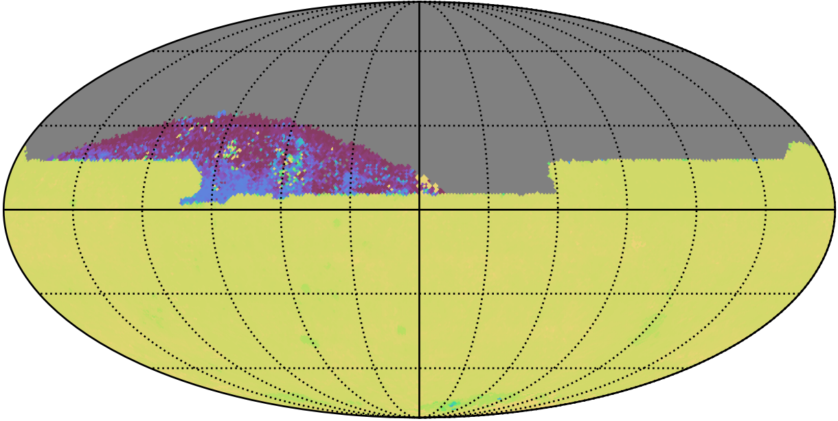
too_elab_heavy_r64_d3_ugrizy_v3.4_10yrs All sky zy bands: 75th Percentile Intranight Timespan
