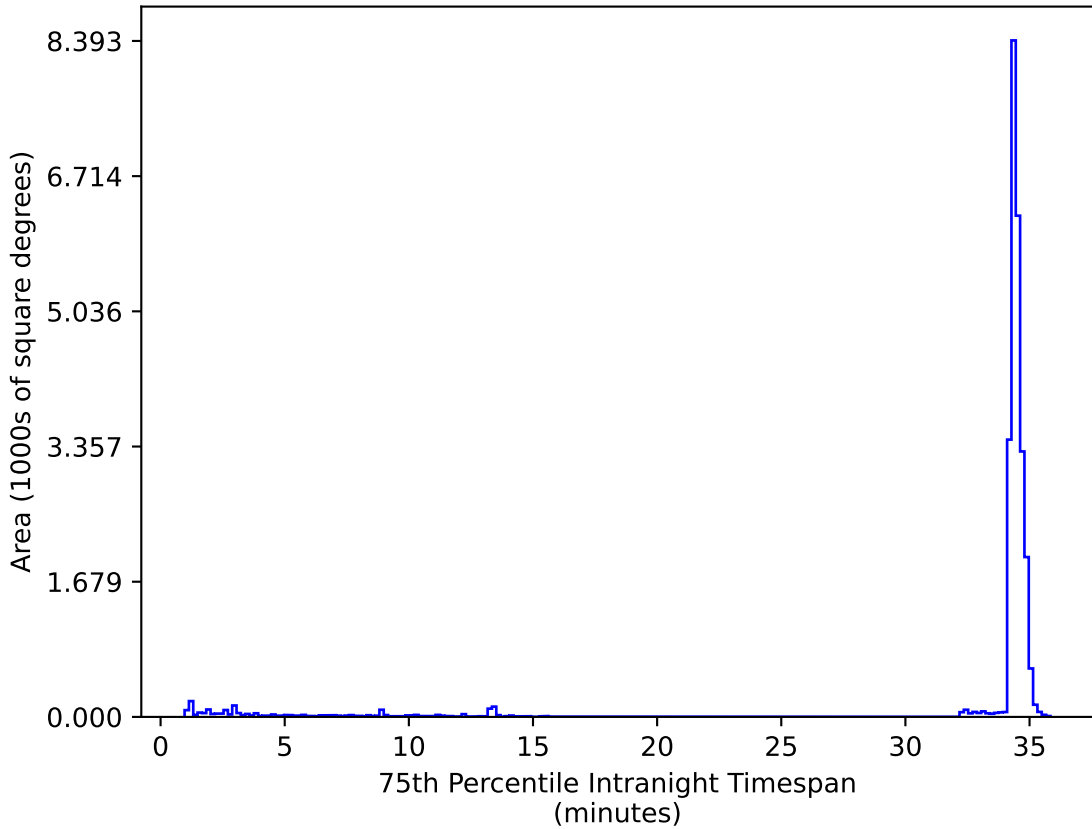
too_elab_heavy_r64_d3_ugrizy_v3.4_10yrs All sky zy bands: 75th Percentile Intranight Timespan
