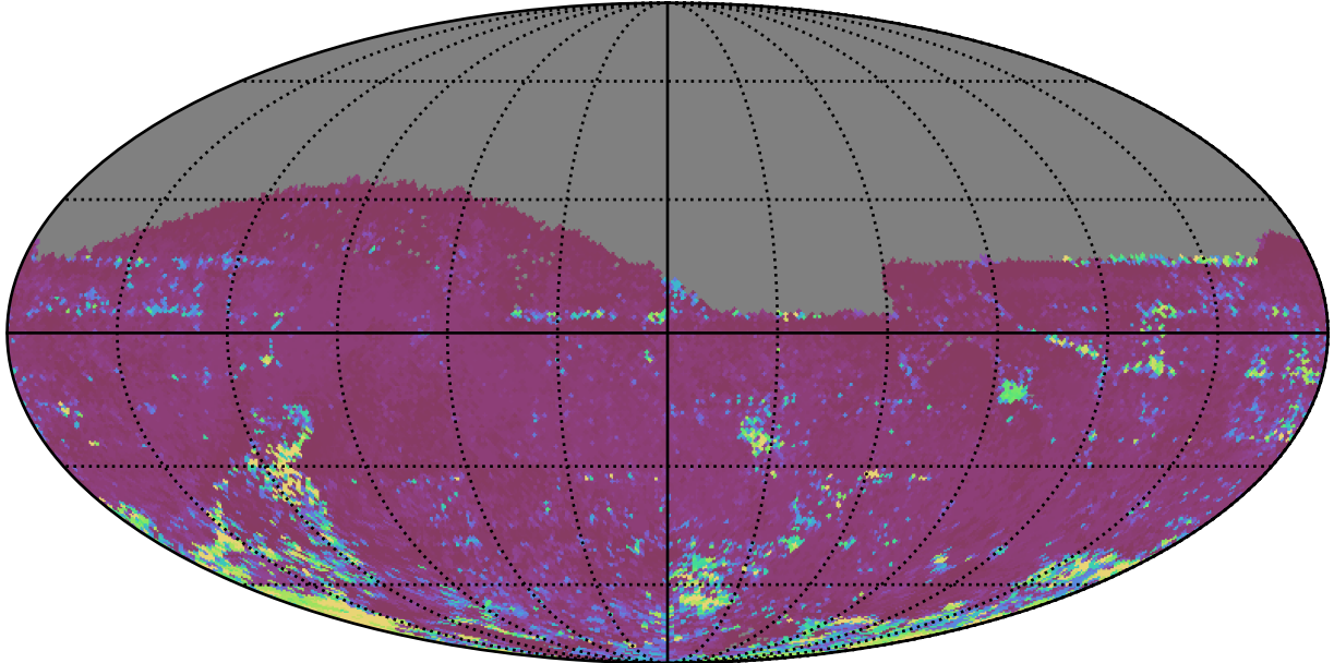
too_elab_heavy_r64_d3_ugrizy_v3.4_10yrs All sky z band: 75th Percentile Intranight Timespan
