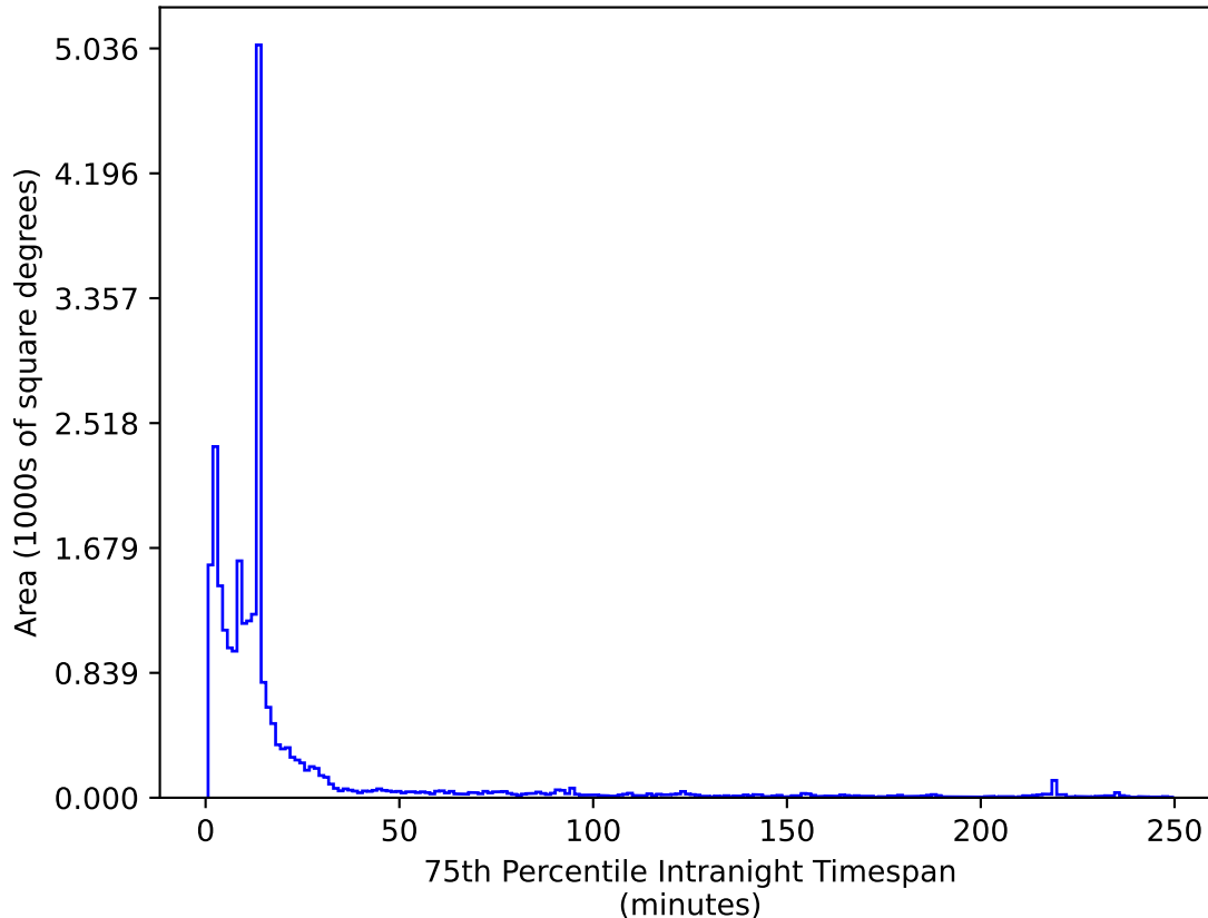
too_elab_heavy_r64_d3_ugrizy_v3.4_10yrs All sky z band: 75th Percentile Intranight Timespan
