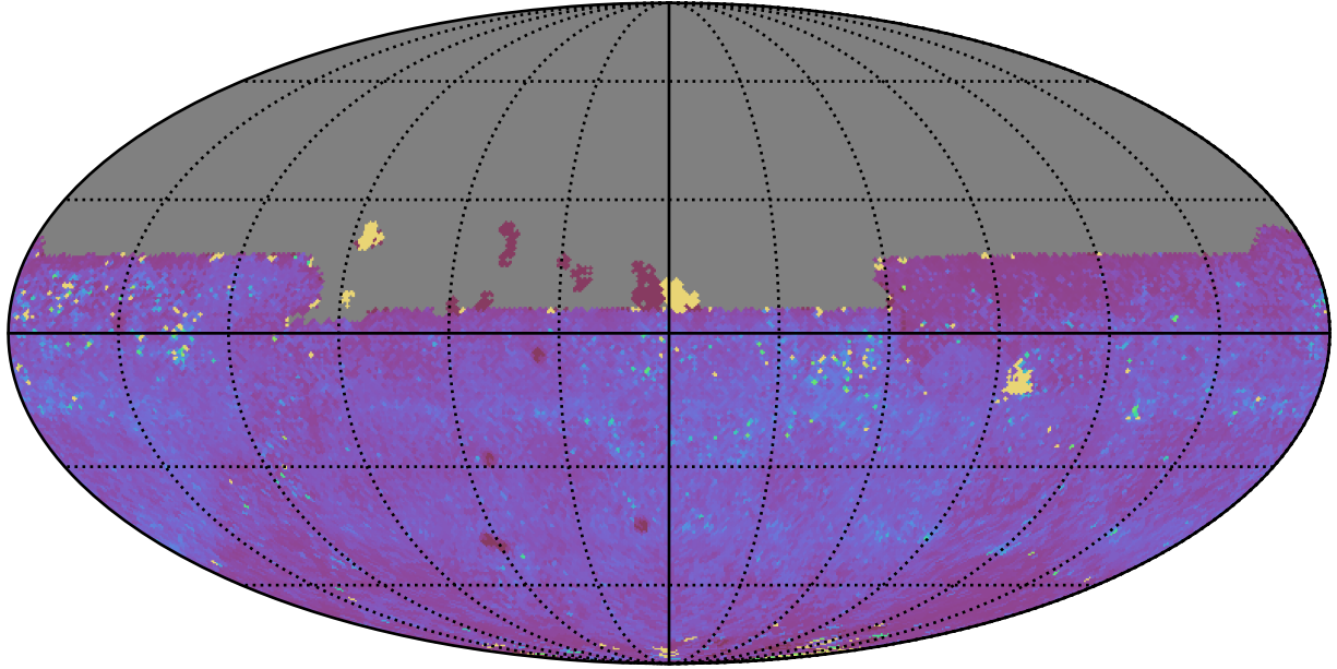
too_elab_heavy_r64_d3_ugrizy_v3.4_10yrs All sky y band: 75th Percentile Intranight Timespan
