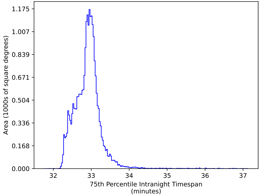
too_elab_heavy_r64_d3_ugrizy_v3.4_10yrs All sky y band: 75th Percentile Intranight Timespan
