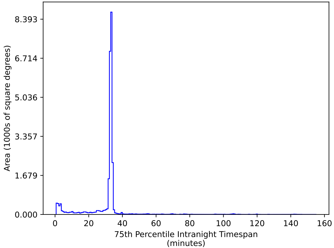
too_elab_heavy_r64_d3_ugrizy_v3.4_10yrs All sky ug bands: 75th Percentile Intranight Timespan
