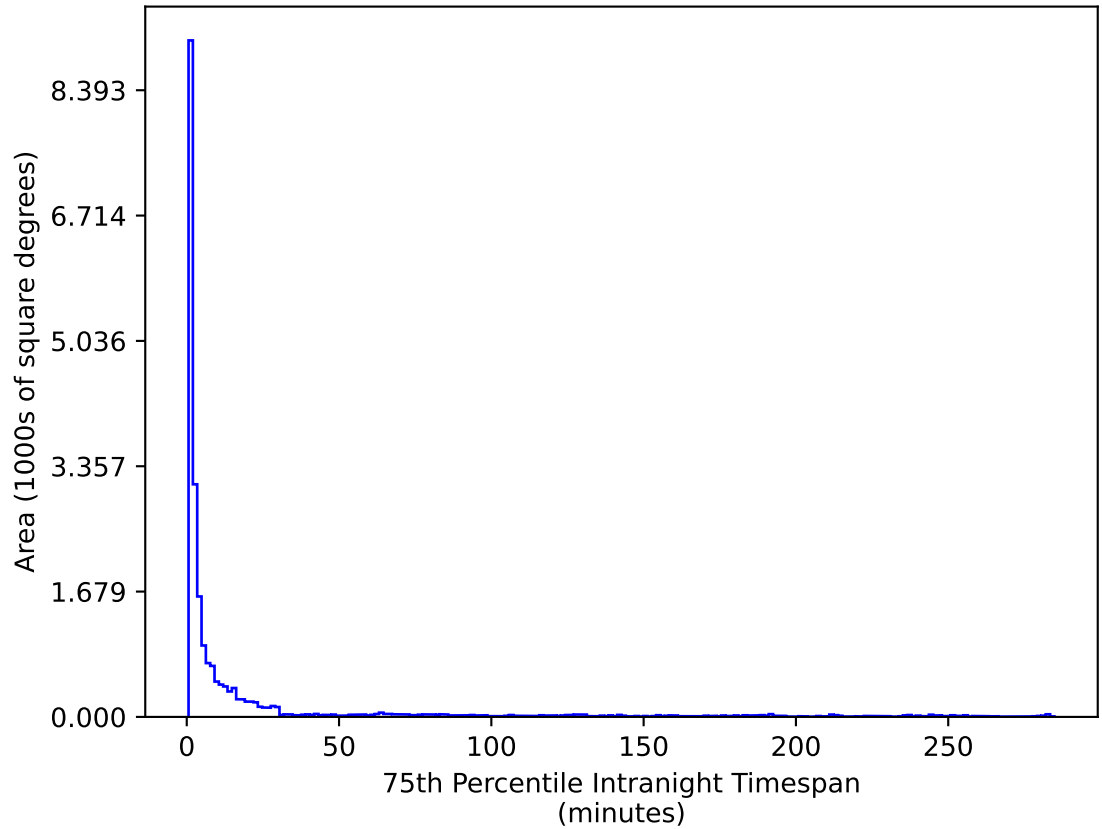
too_elab_heavy_r64_d3_ugrizy_v3.4_10yrs All sky u band: 75th Percentile Intranight Timespan
