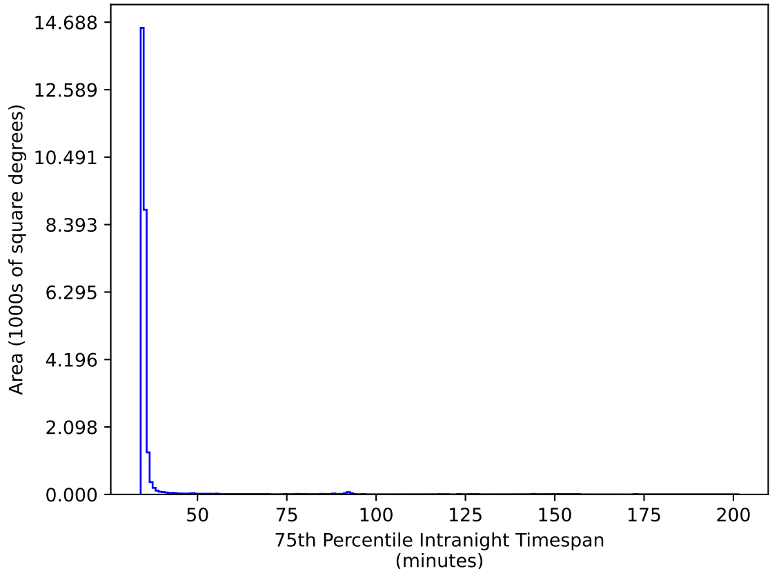
too_elab_heavy_r64_d3_ugrizy_v3.4_10yrs All sky ri bands: 75th Percentile Intranight Timespan
