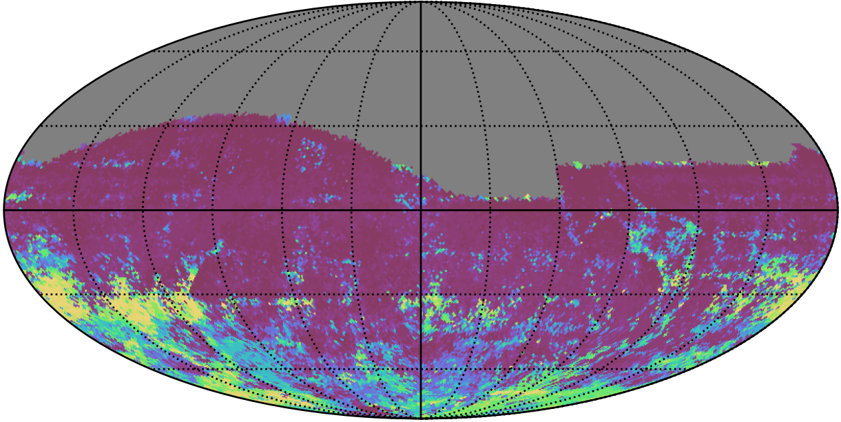
too_elab_heavy_r64_d3_ugrizy_v3.4_10yrs All sky r band: 75th Percentile Intranight Timespan
