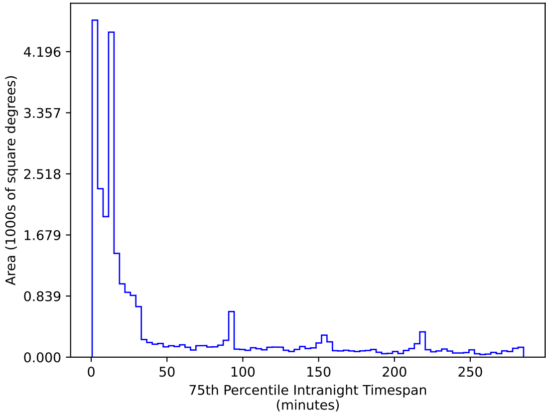
too_elab_heavy_r64_d3_ugrizy_v3.4_10yrs All sky r band: 75th Percentile Intranight Timespan
