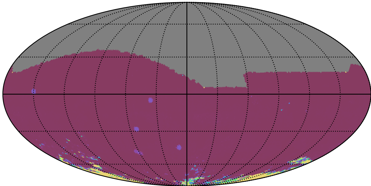
too_elab_heavy_r64_d3_ugrizy_v3.4_10yrs All sky iz bands: 75th Percentile Intranight Timespan
