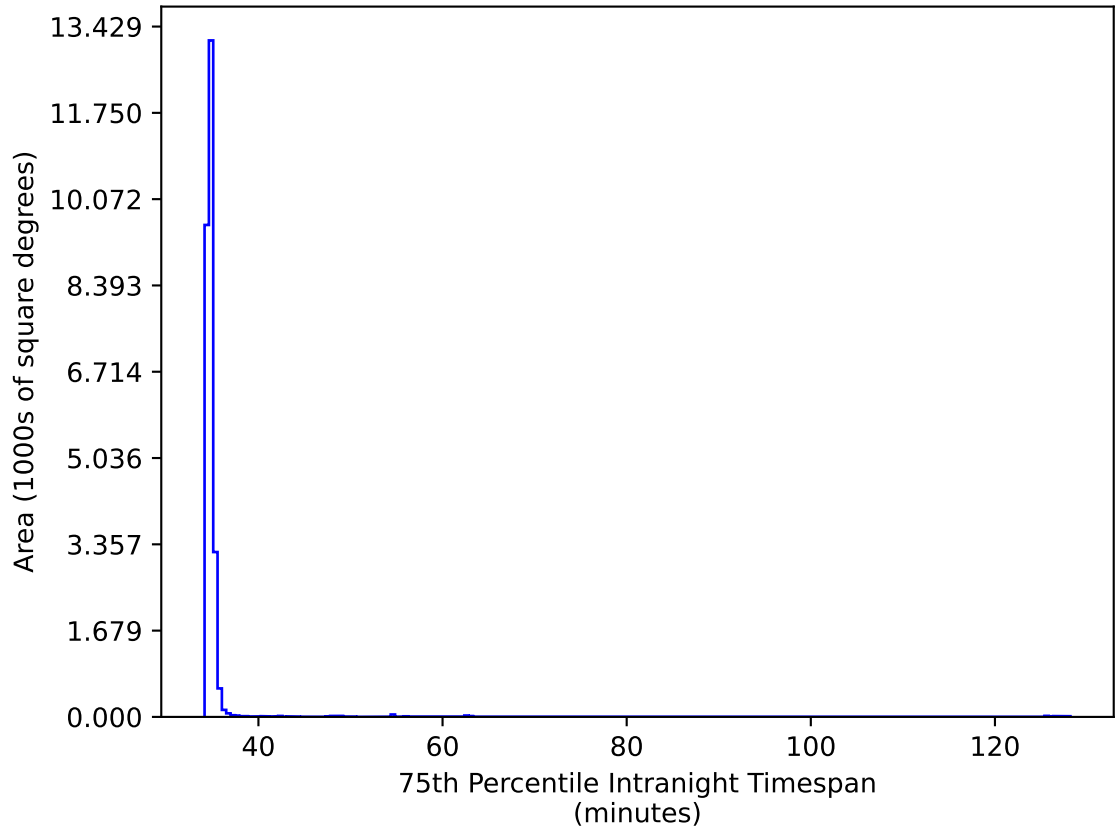
too_elab_heavy_r64_d3_ugrizy_v3.4_10yrs All sky iz bands: 75th Percentile Intranight Timespan
