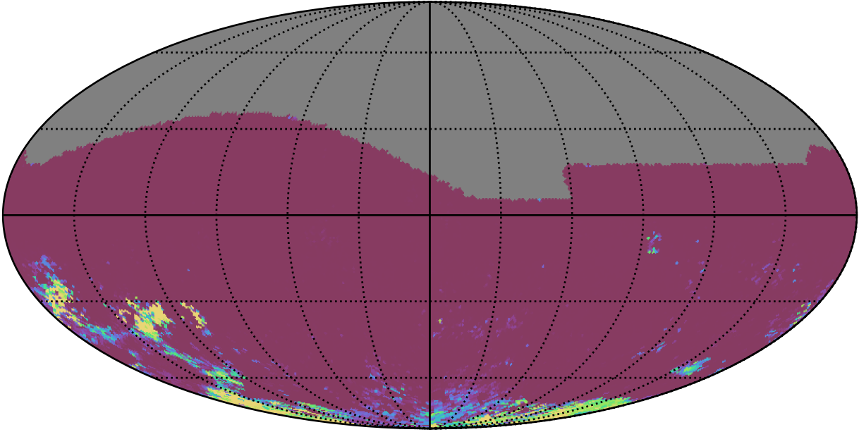
too_elab_heavy_r64_d3_ugrizy_v3.4_10yrs All sky gr bands: 75th Percentile Intranight Timespan
