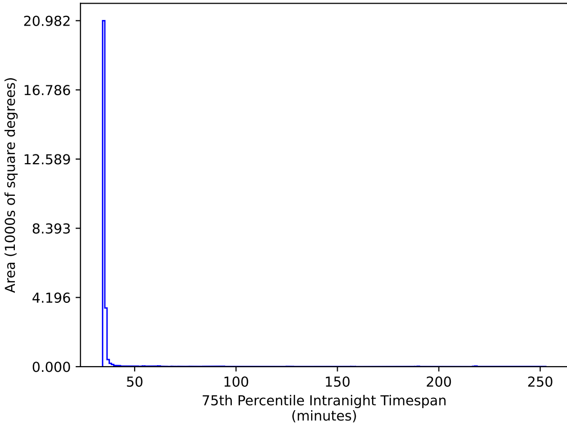
too_elab_heavy_r64_d3_ugrizy_v3.4_10yrs All sky gr bands: 75th Percentile Intranight Timespan
