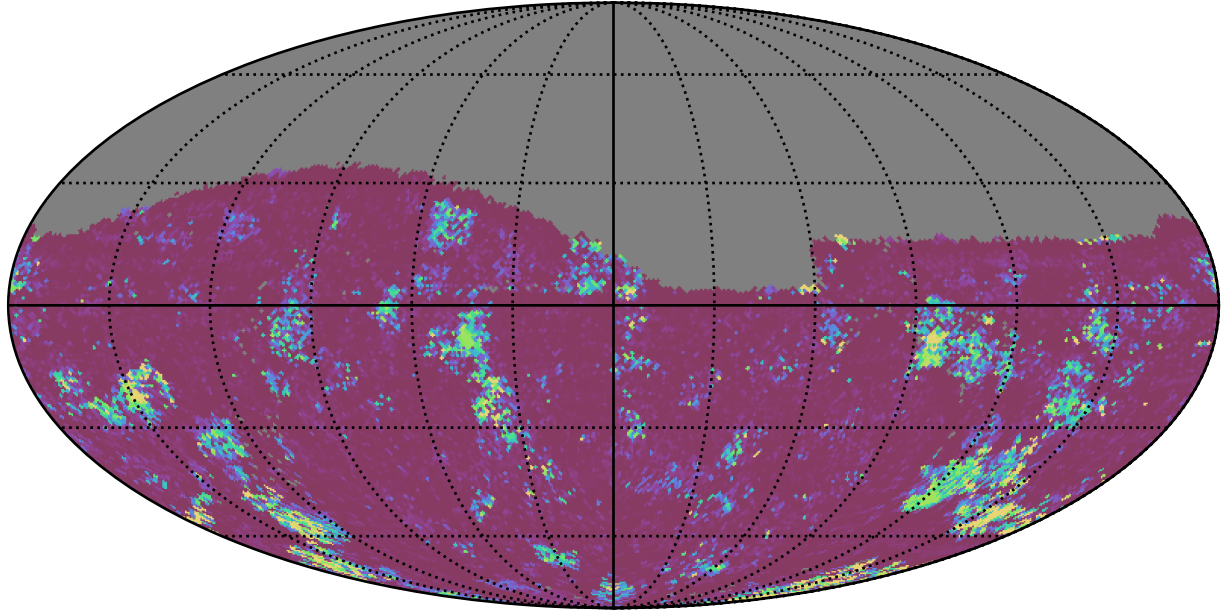
too_elab_heavy_r64_d3_ugrizy_v3.4_10yrs All sky g band: 75th Percentile Intranight Timespan
