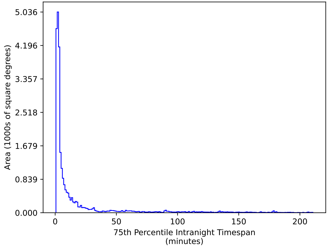
too_elab_heavy_r64_d3_ugrizy_v3.4_10yrs All sky g band: 75th Percentile Intranight Timespan
