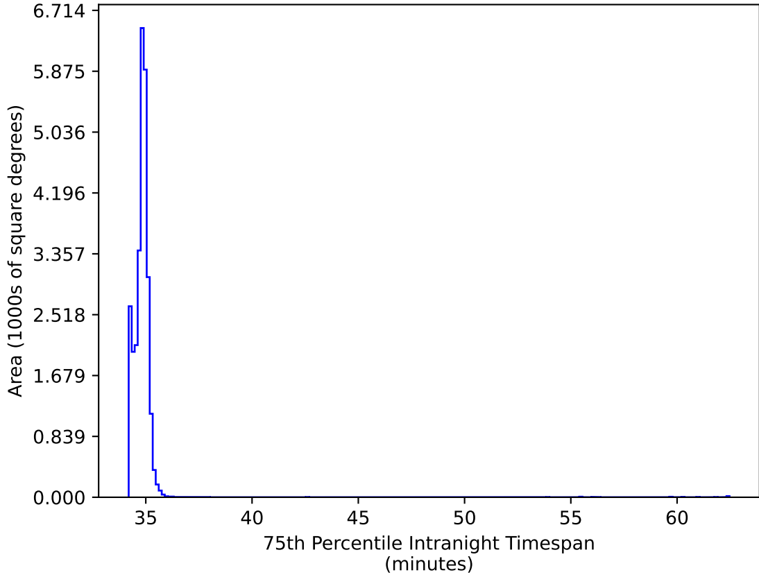
too_elab_heavy_r64_d3_ugrizy_v3.4_10yrs All sky all bands: 75th Percentile Intranight Timespan
