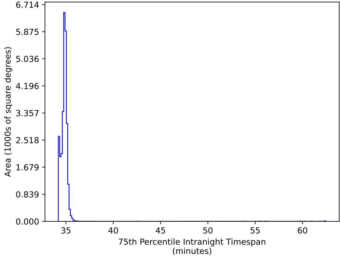
too_elab_heavy_r64_d3_ugrizy_v3.4_10yrs All sky: 75th Percentile Intranight Timespan
