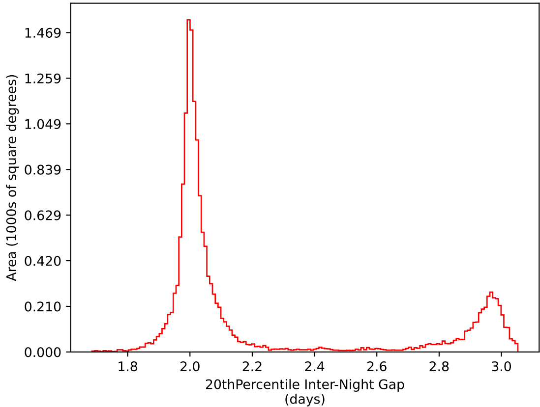
too_elab_heavy_r64_d3_ugrizy_v3.4_10yrs WFD i band: 20thPercentile Inter-Night Gap
