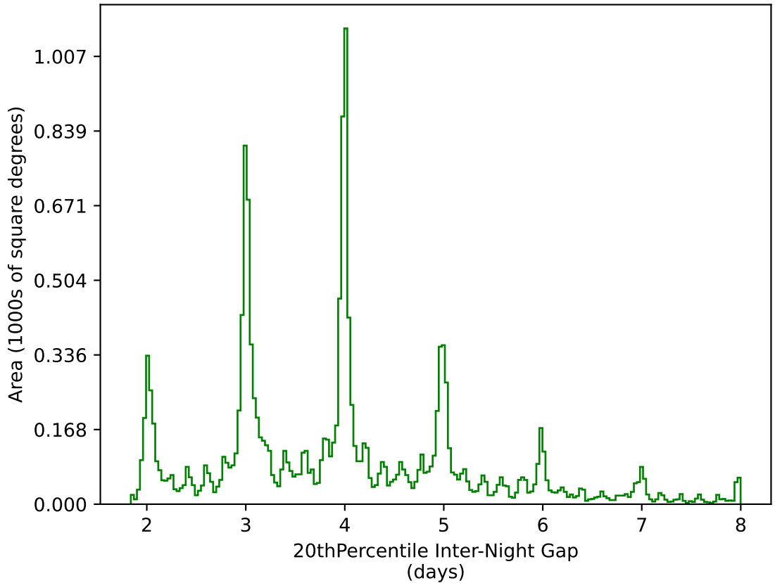
too_elab_heavy_r64_d3_ugrizy_v3.4_10yrs WFD g band: 20thPercentile Inter-Night Gap
