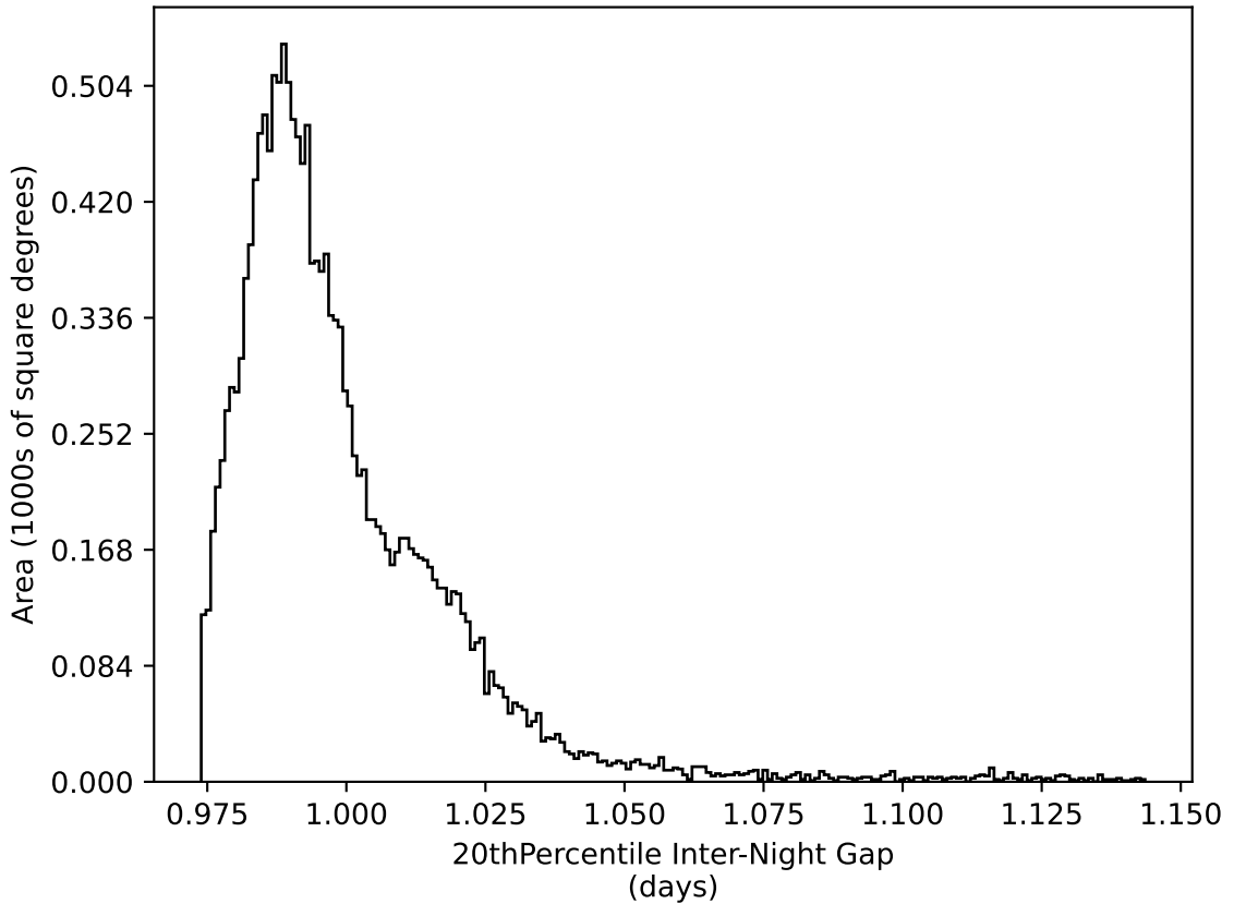
too_elab_heavy_r64_d3_ugrizy_v3.4_10yrs WFD all bands: 20thPercentile Inter-Night Gap
