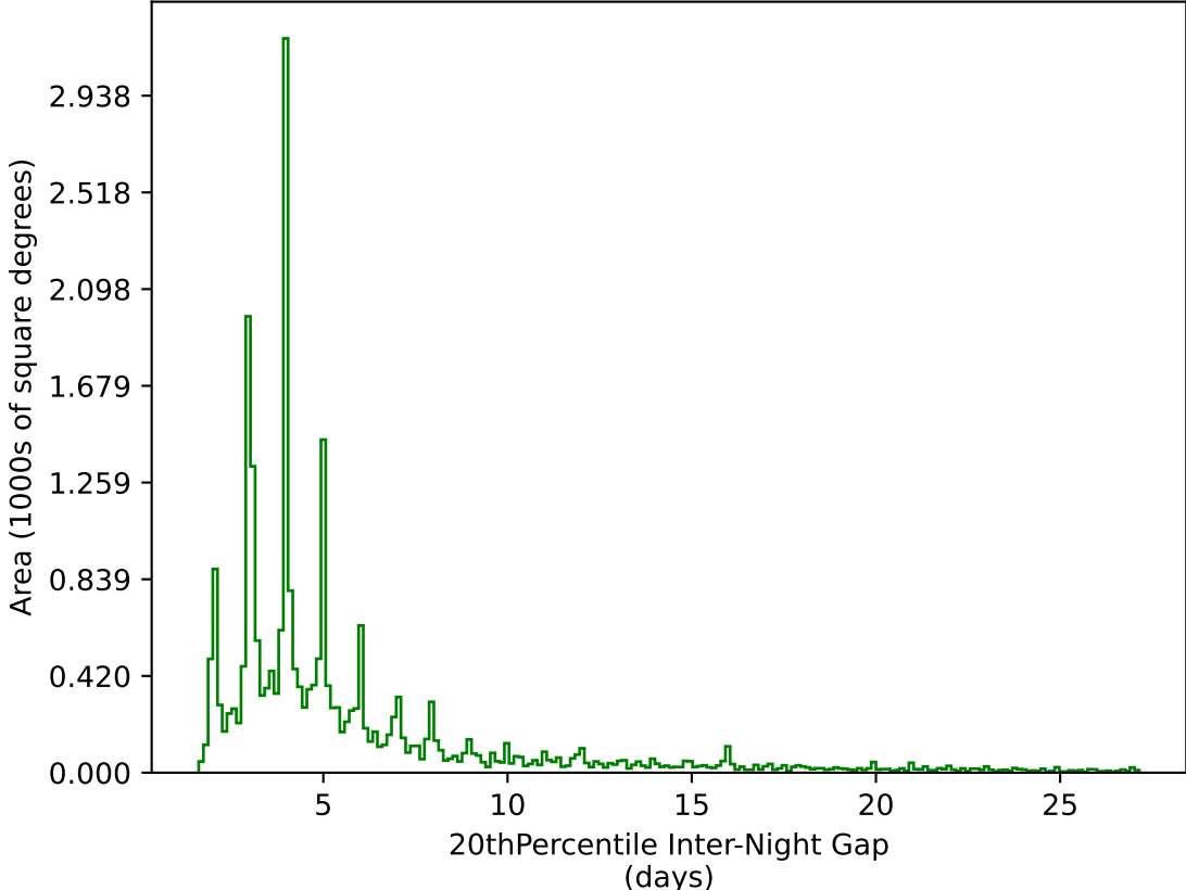
too_elab_heavy_r64_d3_ugrizy_v3.4_10yrs All sky g band: 20thPercentile Inter-Night Gap
