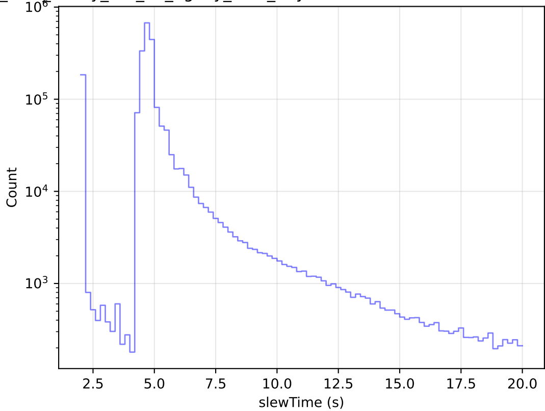
too_elab_heavy_r64_d3_ugrizy_v3.4_10yrs All visits: Zoom Slew Time Histogram
