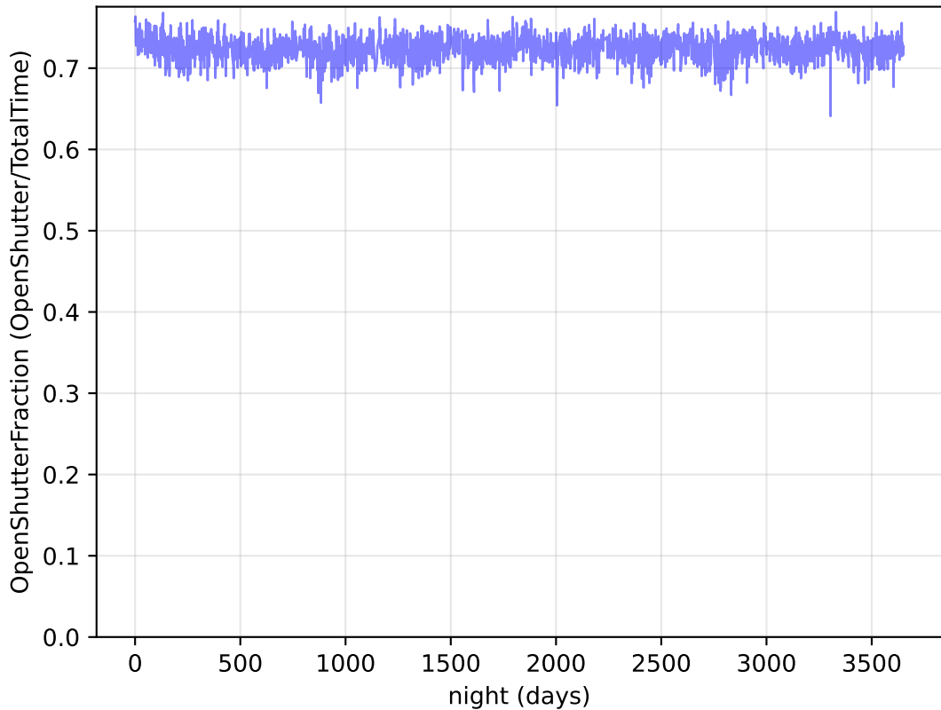
too_elab_heavy_r64_d3_ugrizy_v3.4_10yrs : OpenShutterFraction
