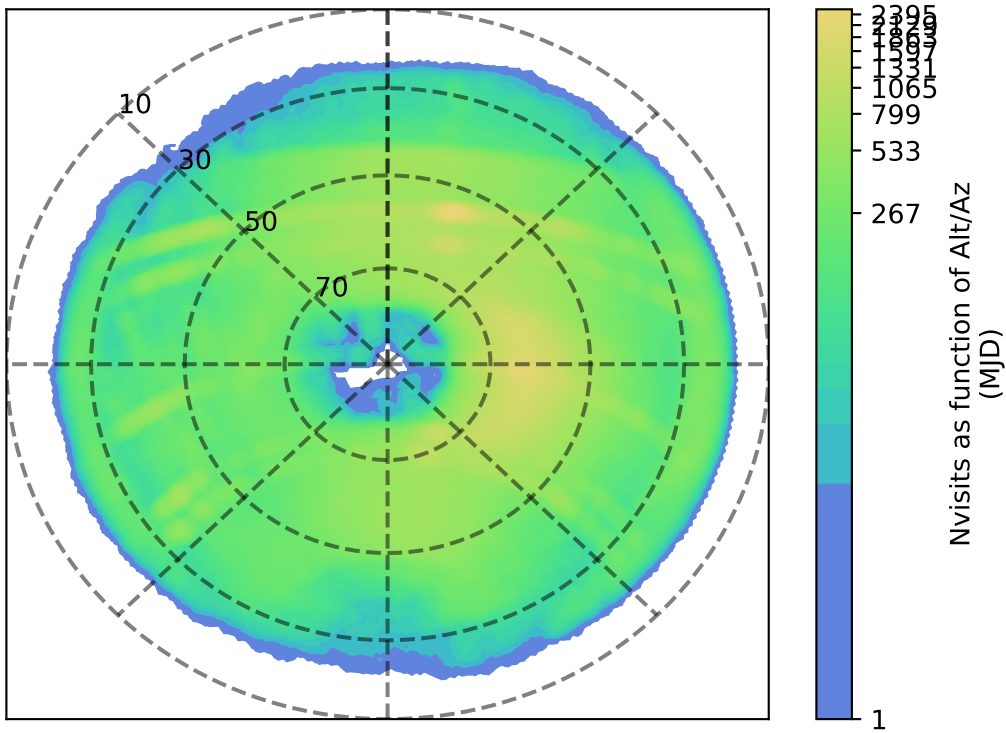
too_elab_heavy_r64_d3_ugrizy_v3.4_10yrs z: Nvisits as function of Alt/Az
