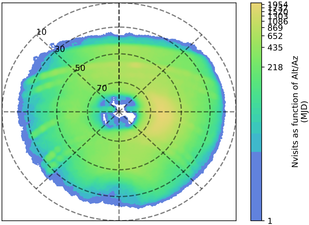
too_elab_heavy_r64_d3_ugrizy_v3.4_10yrs y: Nvisits as function of Alt/Az
