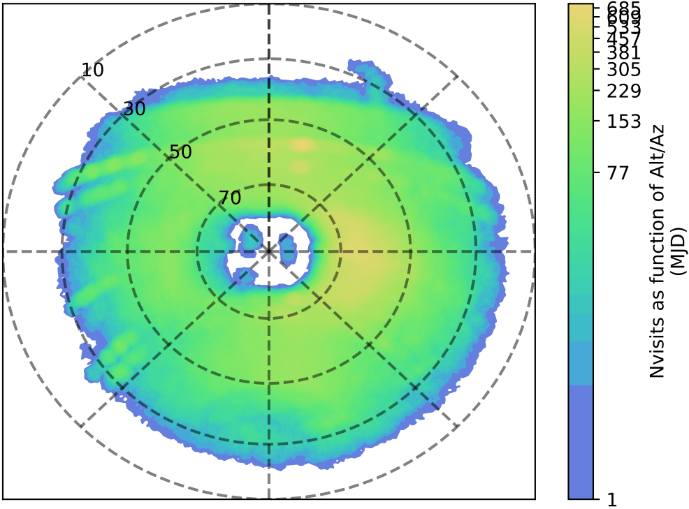
too_elab_heavy_r64_d3_ugrizy_v3.4_10yrs u: Nvisits as function of Alt/Az
