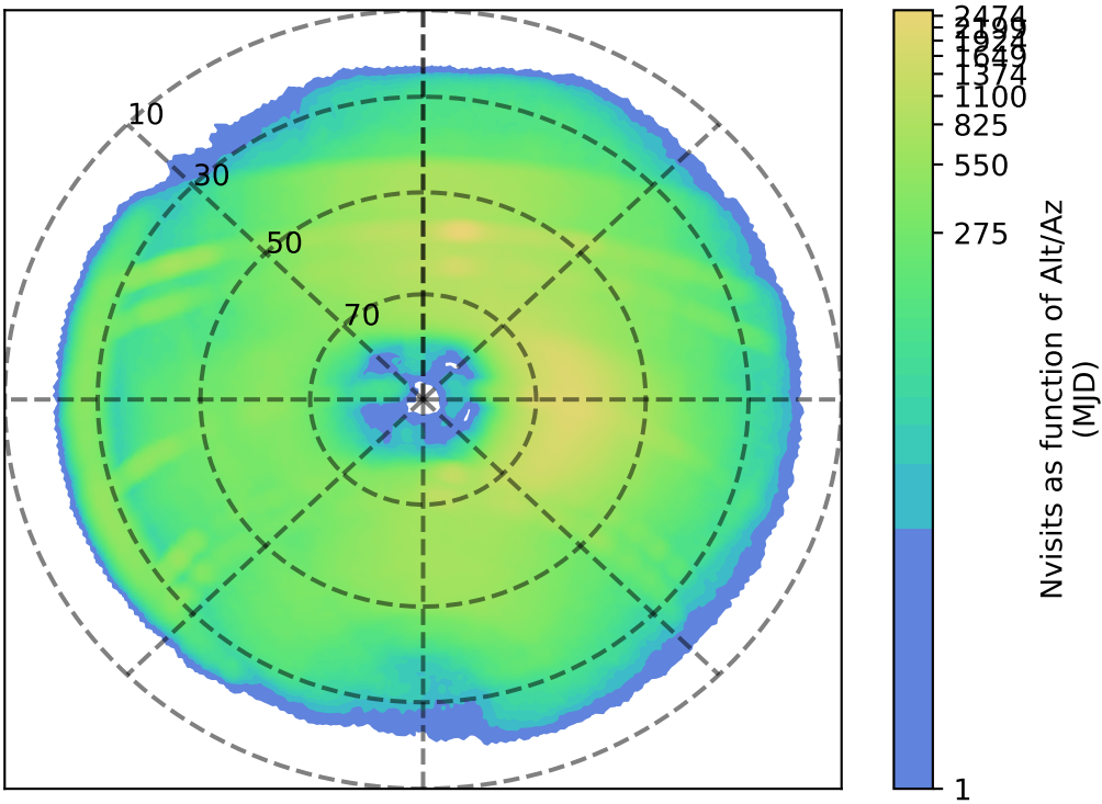
too_elab_heavy_r64_d3_ugrizy_v3.4_10yrs r: Nvisits as function of Alt/Az
