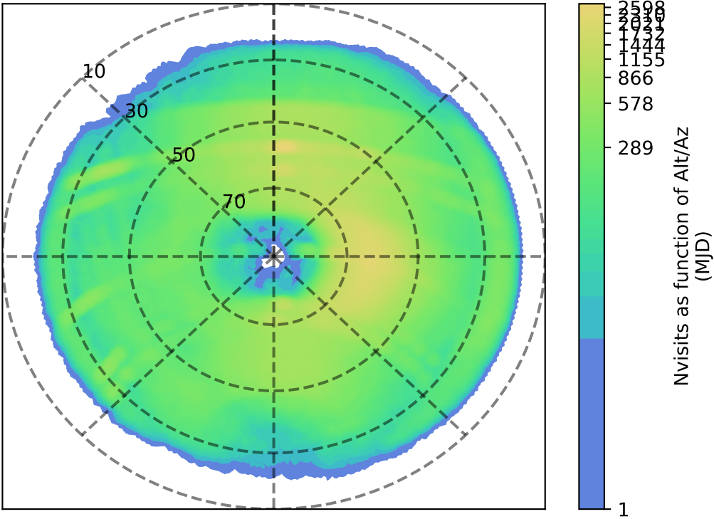
too_elab_heavy_r64_d3_ugrizy_v3.4_10yrs i: Nvisits as function of Alt/Az
