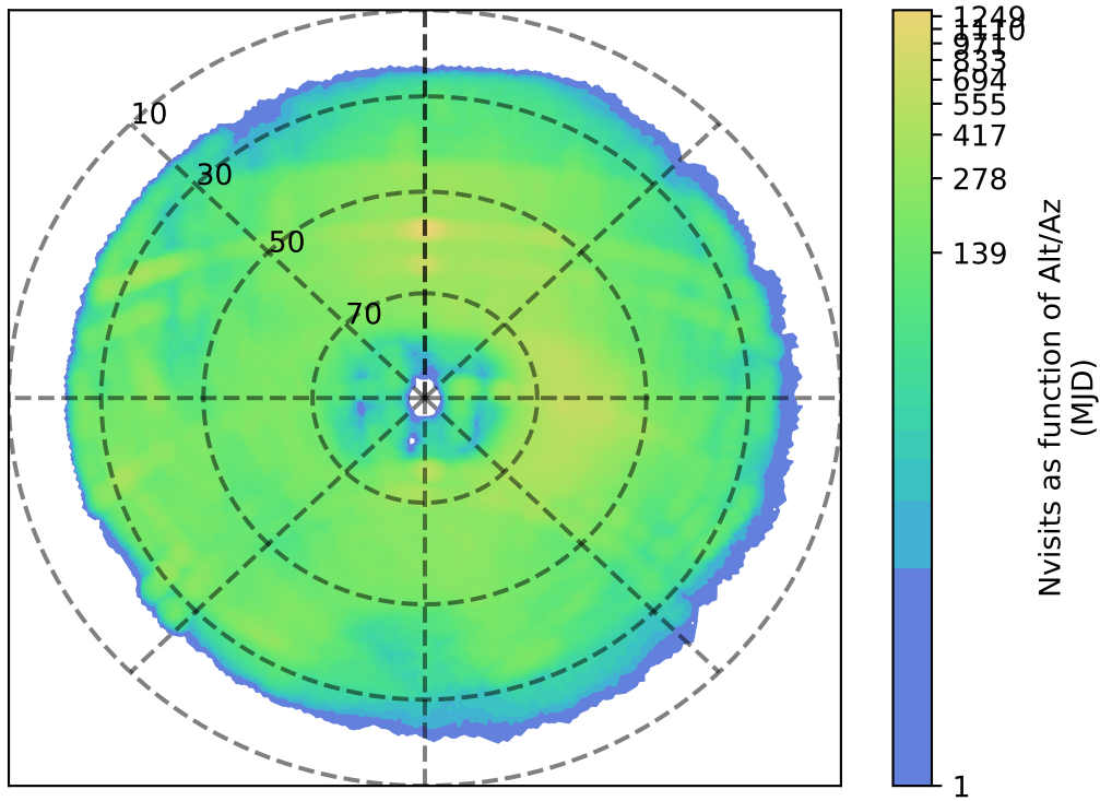
too_elab_heavy_r64_d3_ugrizy_v3.4_10yrs g: Nvisits as function of Alt/Az
