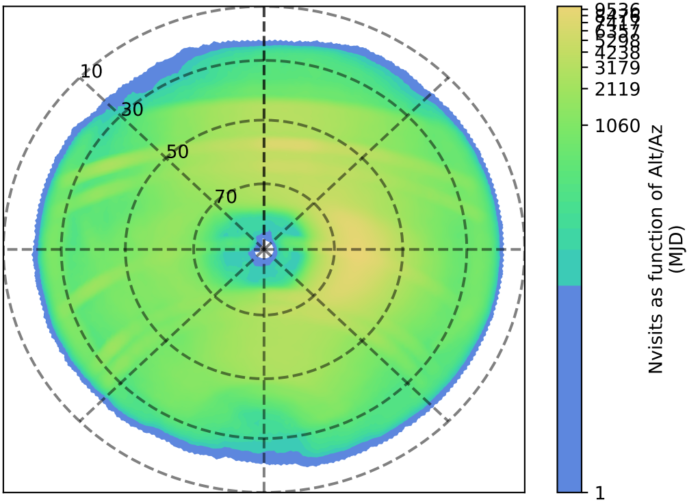
too_elab_heavy_r64_d3_ugrizy_v3.4_10yrs : Nvisits as function of Alt/Az
