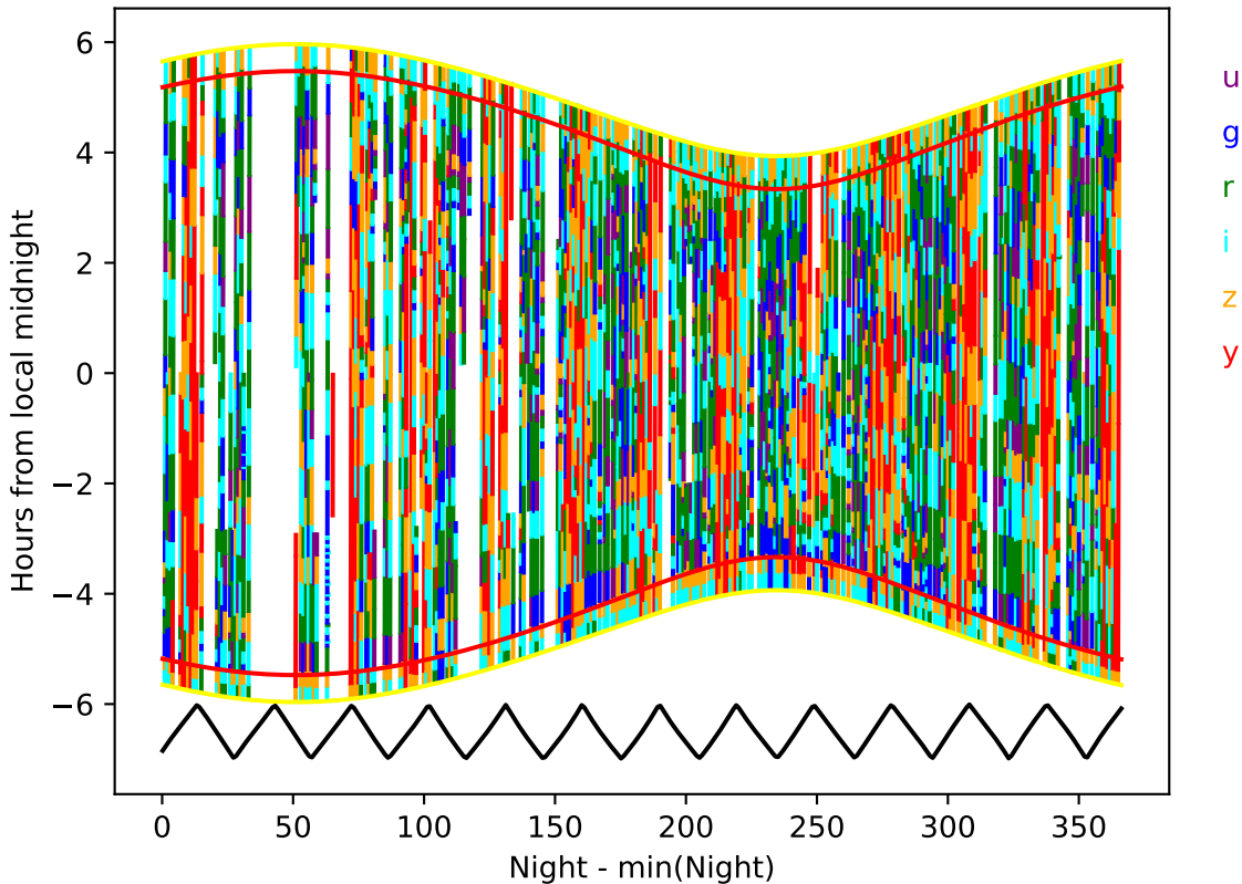
too_elab_heavy_r64_d3_ugrizy_v3.4_10yrs year 8-9: Hourglass
