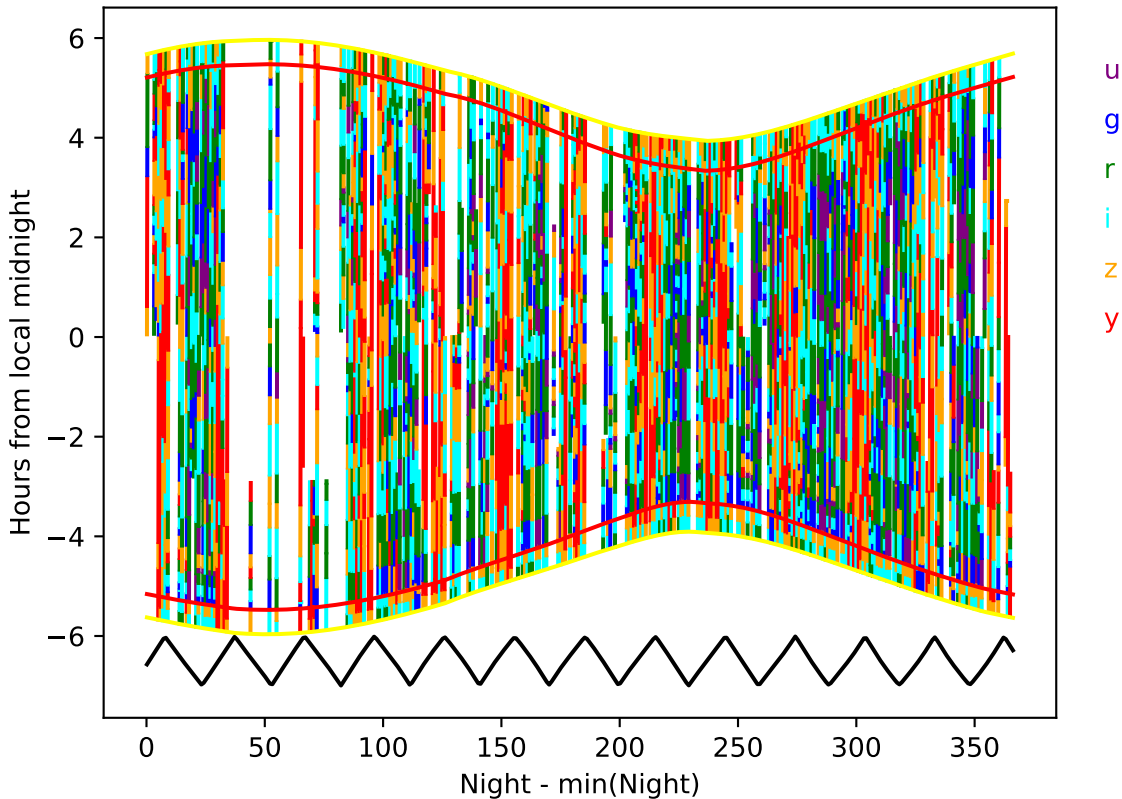
too_elab_heavy_r64_d3_ugrizy_v3.4_10yrs year 3-4: Hourglass
