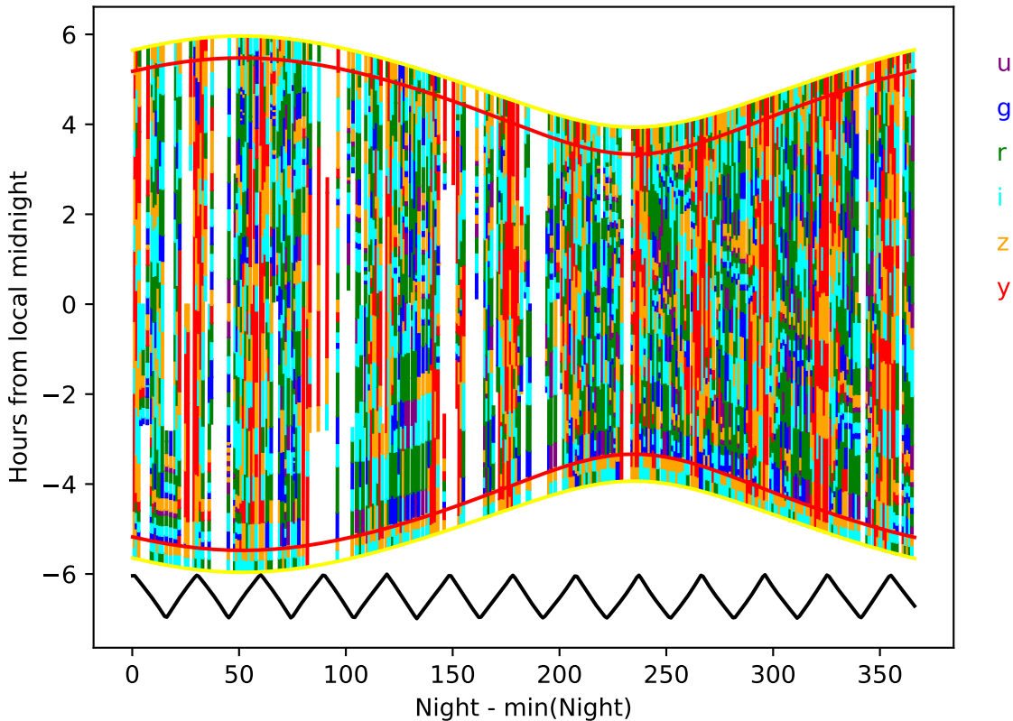
too_elab_heavy_r64_d3_ugrizy_v3.4_10yrs year 1-2: Hourglass
