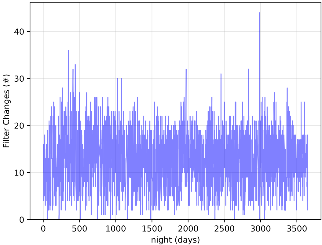
too_elab_heavy_r64_d3_ugrizy_v3.4_10yrs : Filter Changes
