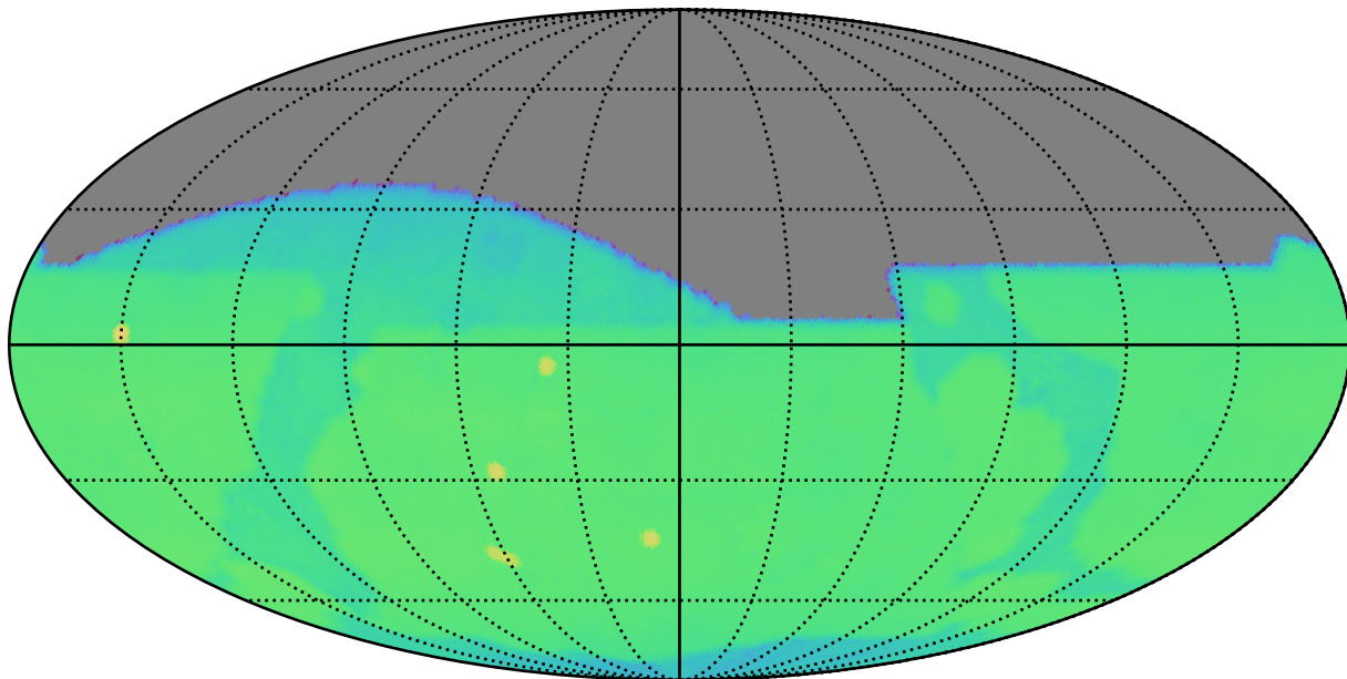
too_elab_heavy_r64_d3_ugrizy_v3.4_10yrs : CoaddM5
