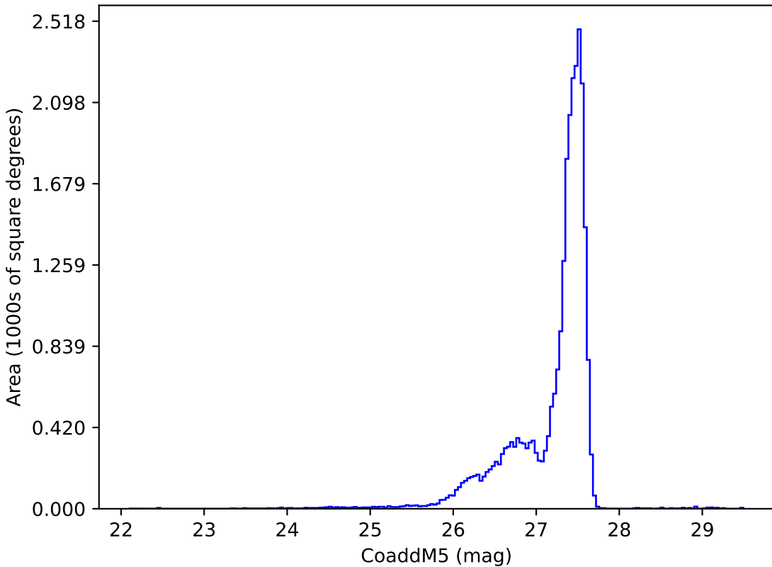
too_elab_heavy_r64_d3_ugrizy_v3.4_10yrs : CoaddM5
