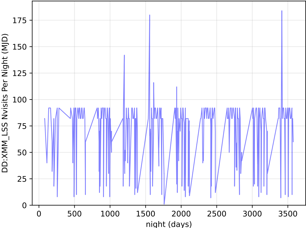
too_elab_heavy_r64_d3_ugrizy_v3.4_10yrs all bands: DD:XMM_LSS Nvisits Per Night
