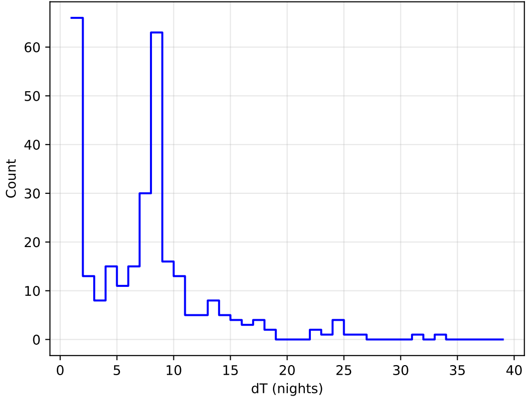
too_elab_heavy_r64_d3_ugrizy_v3.4_10yrs all bands: DD:XMM_LSS Delta Nights Histogram
