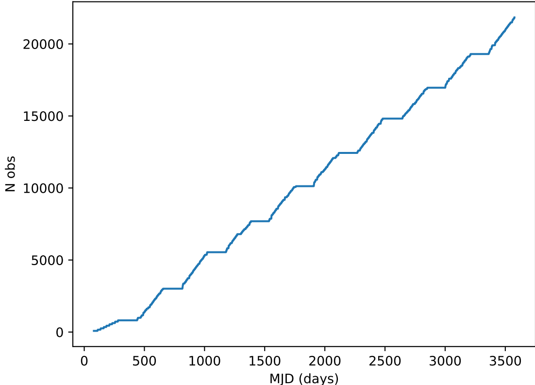
too_elab_heavy_r64_d3_ugrizy_v3.4_10yrs all bands: DD:XMM_LSS Cumulative NVisits
