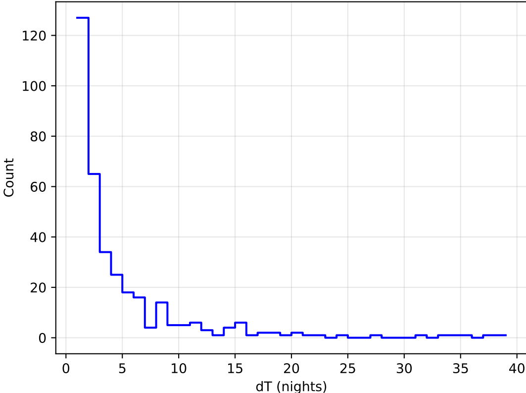
too_elab_heavy_r64_d3_ugrizy_v3.4_10yrs all bands: DD:WFD Delta Nights Histogram
